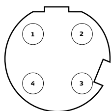
C) M12 hona, 4 stift
