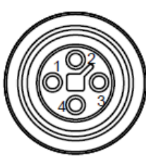
D) M12 hona, 4 stift
