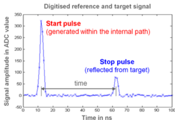
Figure 9 – Measurement principle of the WFD technology.
