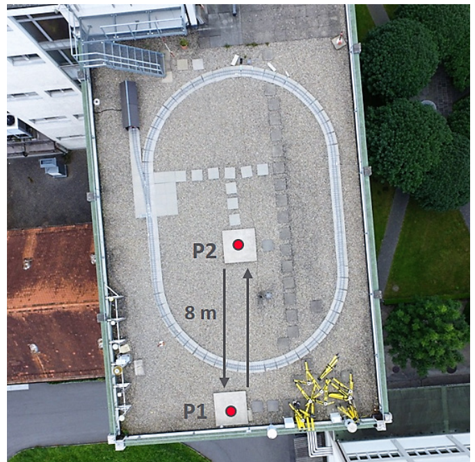
Figure 12 - RTK performance benchmarking under open sky by measuring two points alternately in the instantaneous mode for 10 minutes (Rover A vs. GS18 T, pole length: 1.800 m).
