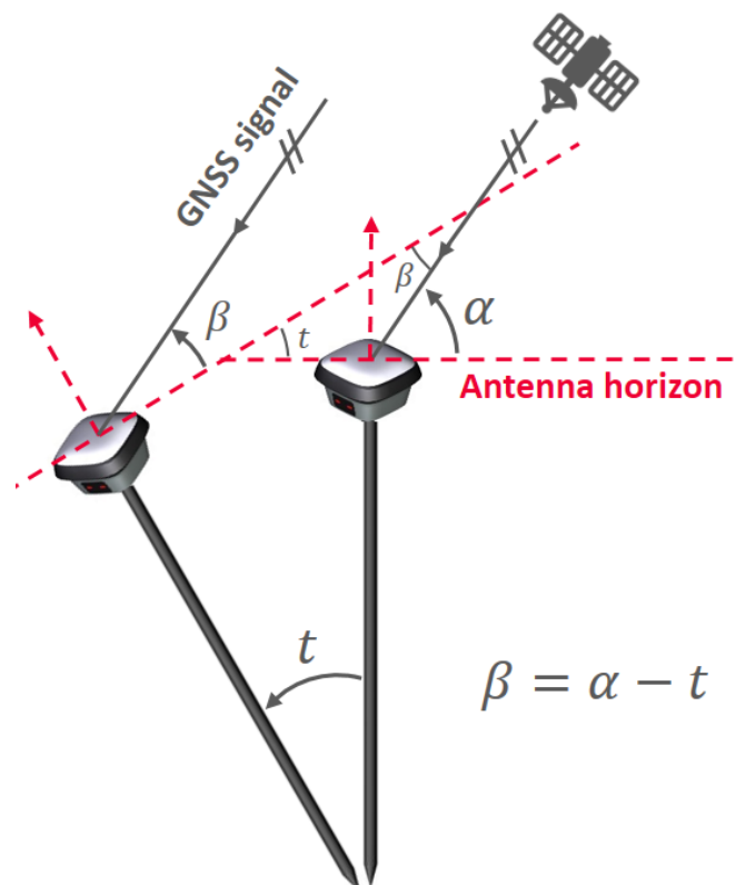
Figure 4 - Decrease in the elevation angle of the incoming GNSS signal when tilting a pole away from satellite ( \alpha : satellite elevation angle for a vertical pole, \beta : satellite elevation angle for a tilted pole, t : tilt angle).
